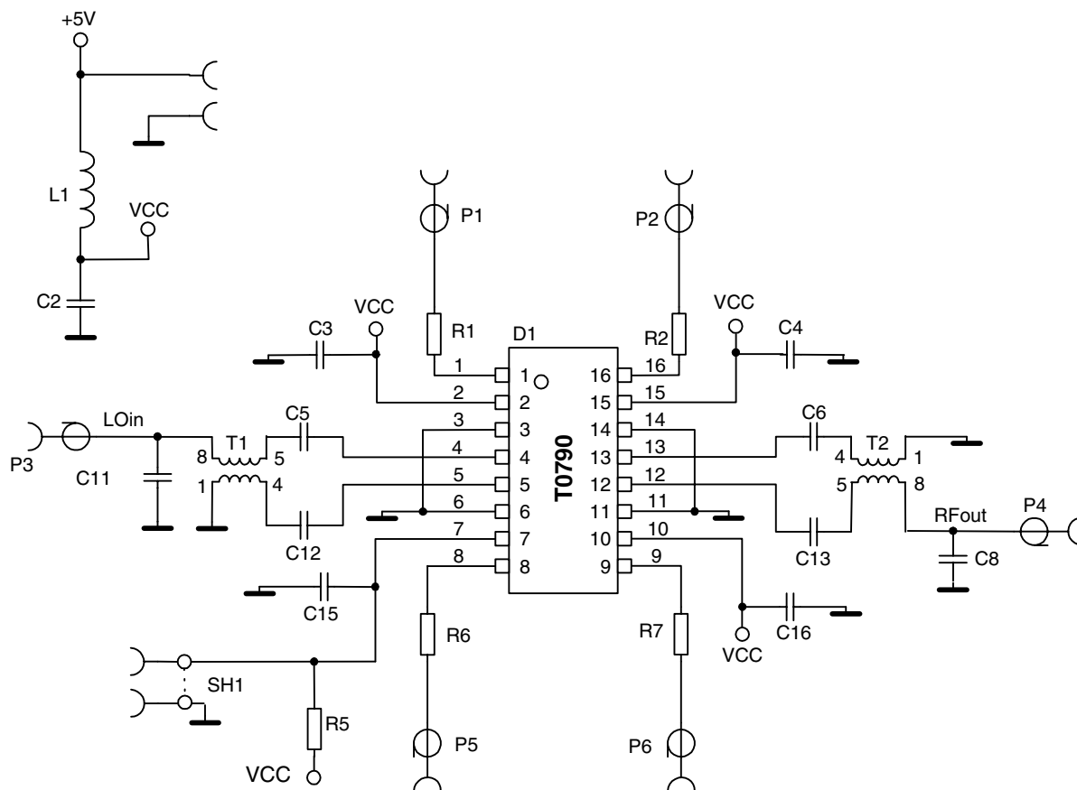
Figure 15. Application Schematic
